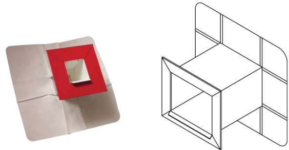
Single Skirt Scupper with Metal Flange
